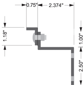
Adjustable handrail bracket
