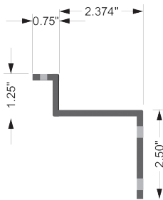
Fixed handrail bracket
